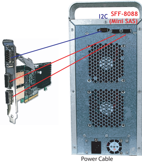
SFF8088 connected to the EditPRO
