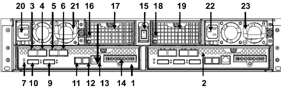
CR-R712FS/D Fiber-SAS/SATA RAID SUBSYSTEM
