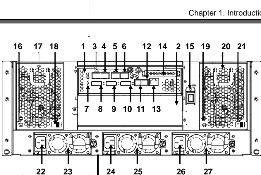
CR-R624SS/D SAS-SAS/SATA RAID SUBSYSTEM
