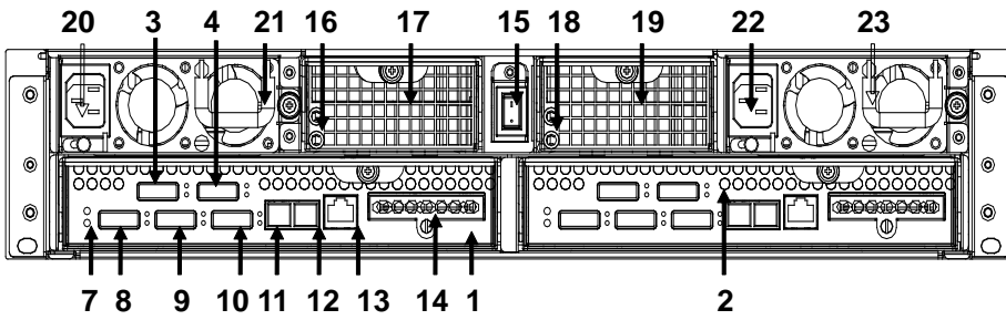
CR-R612SS/D SAS-SAS/SATA RAID SUBSYSTEM
