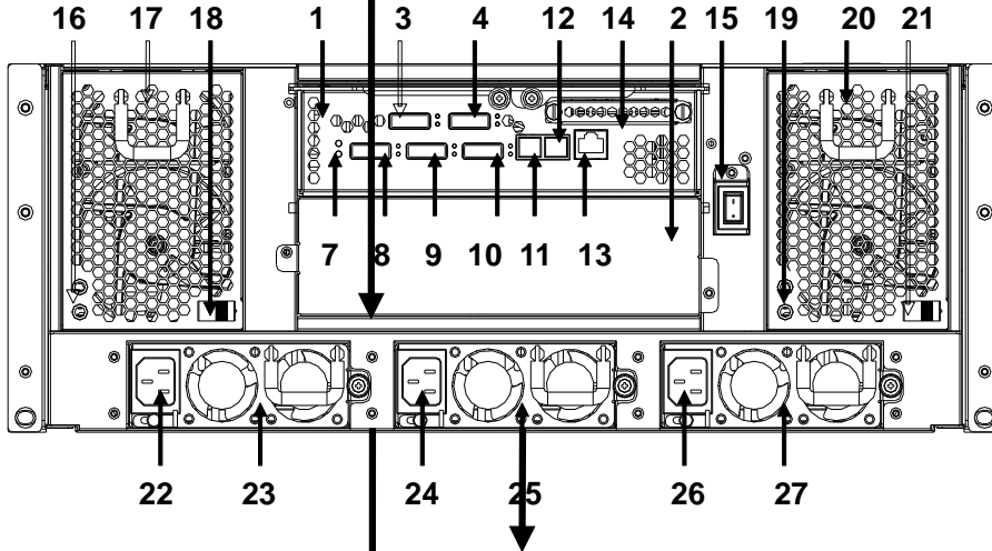
CR-R624SS/D SAS-SAS/SATA RAID SUBSYSTEM
